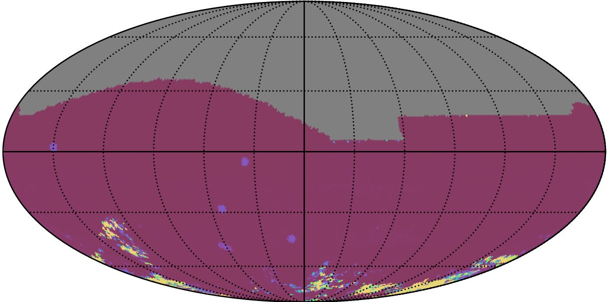
early_u_fpextra2.0_v3.4_10yrs All sky iz bands: 75th Percentile Intranight Timespan
