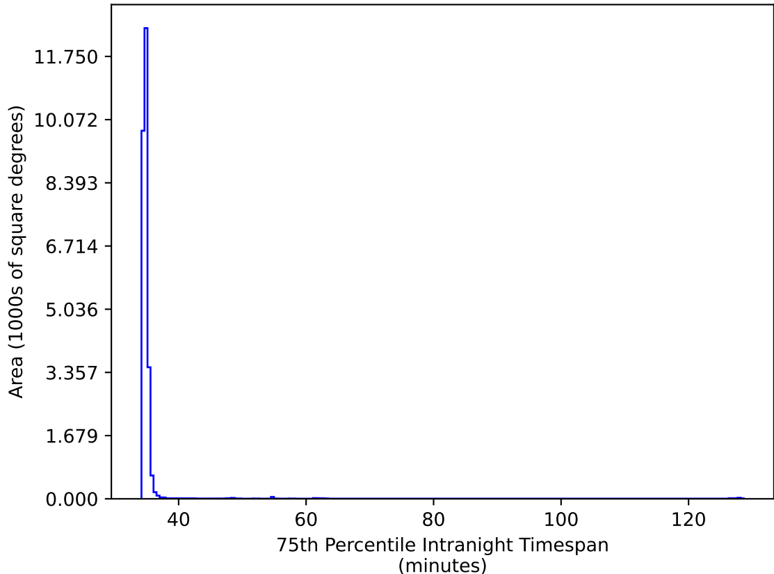
early_u_fpextra2.0_v3.4_10yrs All sky iz bands: 75th Percentile Intranight Timespan
