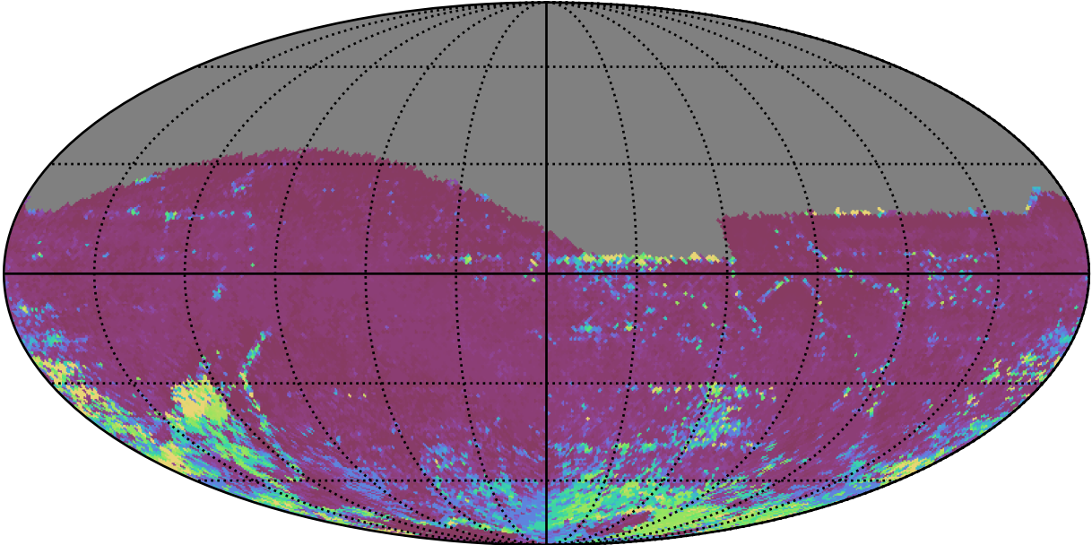
early_u_fpextra2.0_v3.4_10yrs All sky i band: 75th Percentile Intranight Timespan
