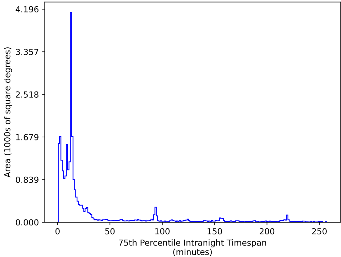
early_u_fpextra2.0_v3.4_10yrs All sky i band: 75th Percentile Intranight Timespan
