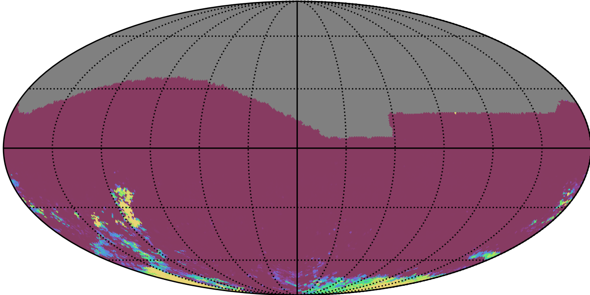
early_u_fpextra2.0_v3.4_10yrs All sky gr bands: 75th Percentile Intranight Timespan
