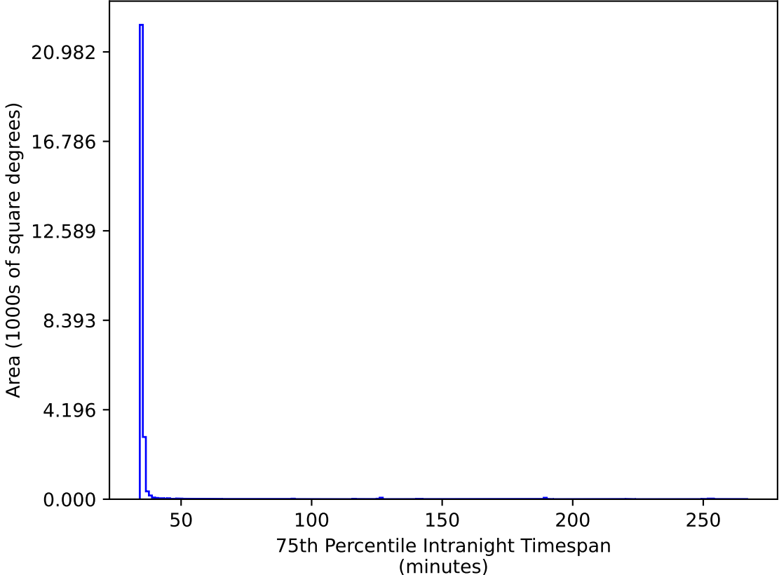
early_u_fpextra2.0_v3.4_10yrs All sky gr bands: 75th Percentile Intranight Timespan
