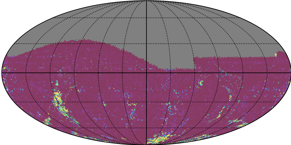
early_u_fpextra2.0_v3.4_10yrs All sky g band: 75th Percentile Intranight Timespan
