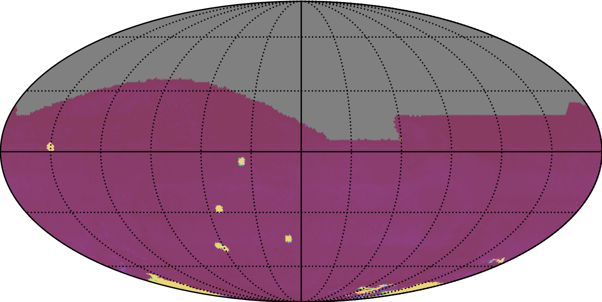
early_u_fpextra2.0_v3.4_10yrs All sky all bands: 75th Percentile Intranight Timespan
