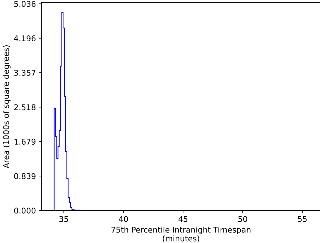
early_u_fpextra2.0_v3.4_10yrs All sky: 75th Percentile Intranight Timespan
