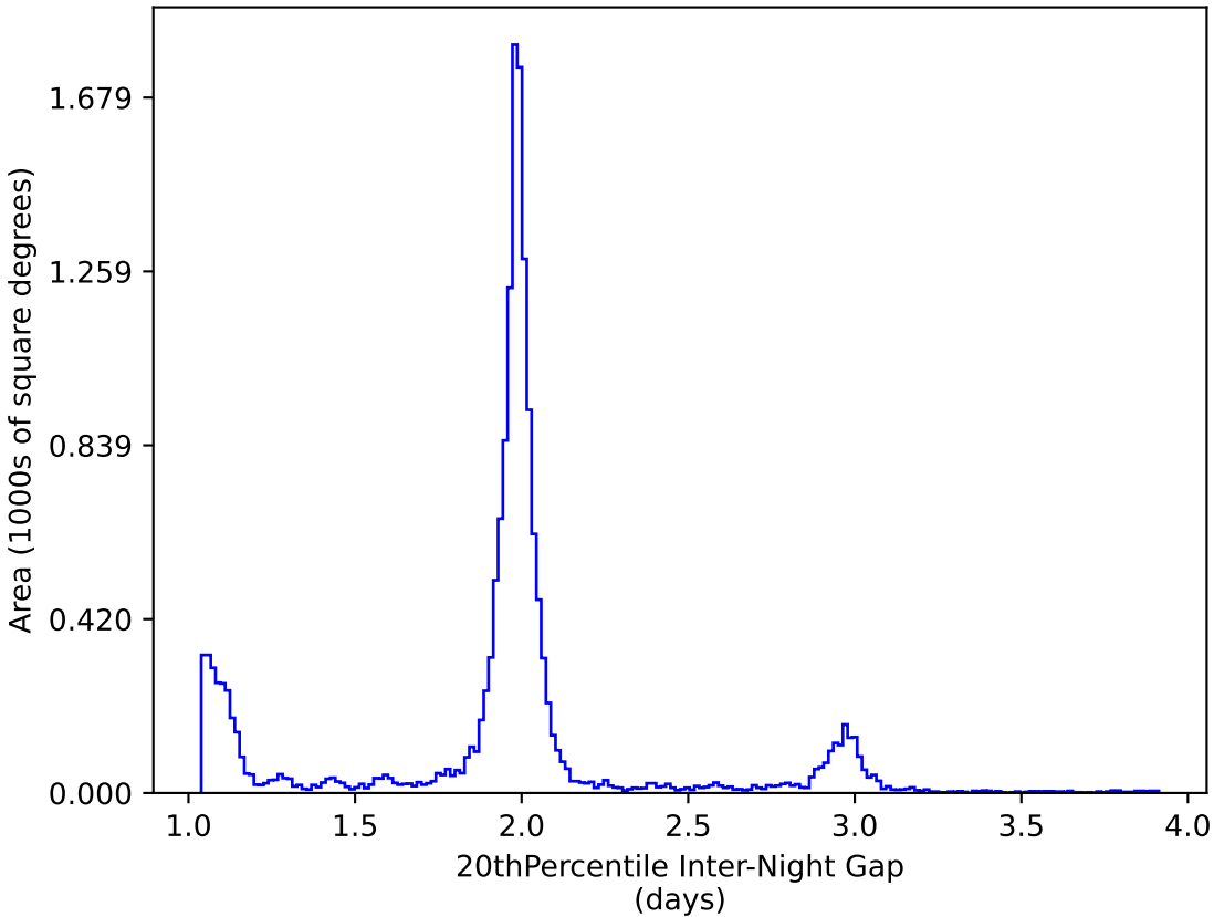
early_u_fpextra2.0_v3.4_10yrs WFD y band: 20thPercentile Inter-Night Gap
