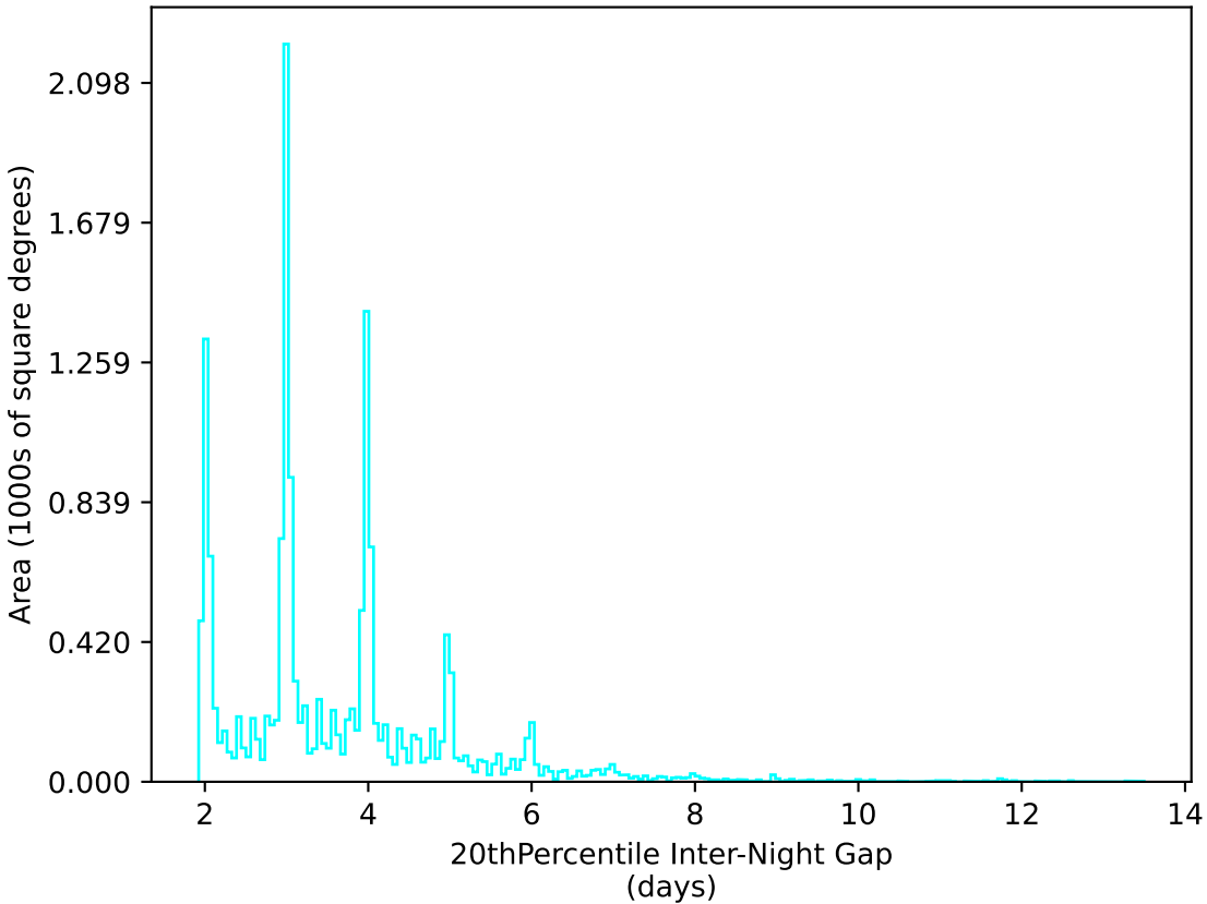
early_u_fpextra2.0_v3.4_10yrs WFD u band: 20thPercentile Inter-Night Gap
