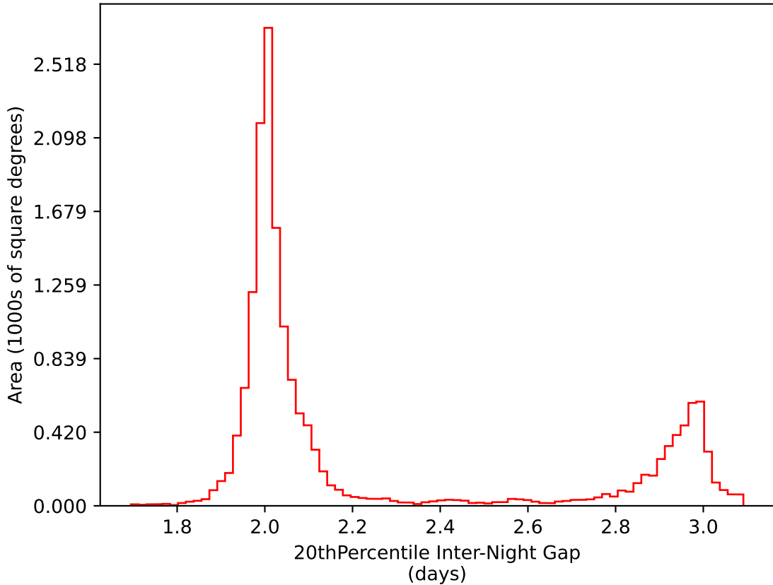
early_u_fpextra2.0_v3.4_10yrs WFD i band: 20thPercentile Inter-Night Gap
