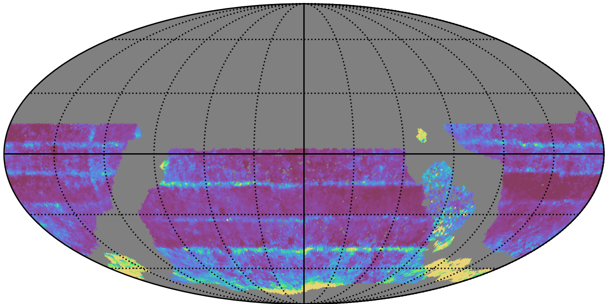
early_u_fpextra2.0_v3.4_10yrs WFD all bands: 20thPercentile Inter-Night Gap
