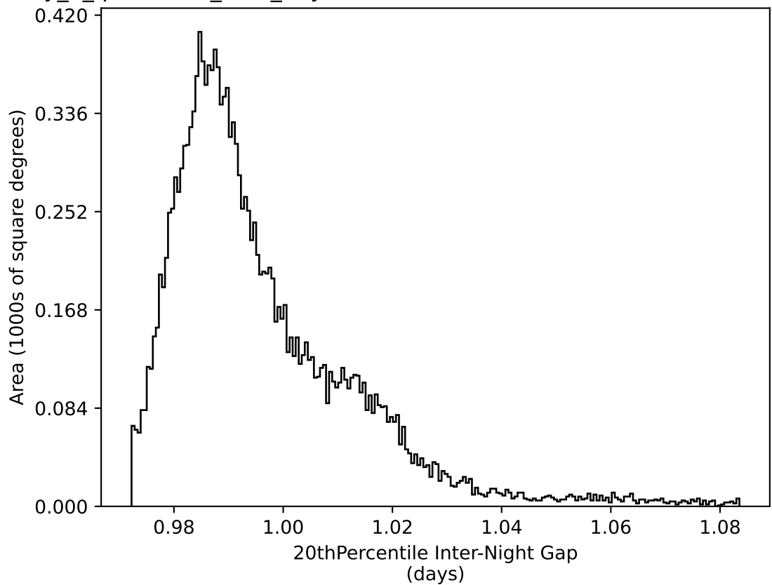
early_u_fpextra2.0_v3.4_10yrs WFD all bands: 20thPercentile Inter-Night Gap
