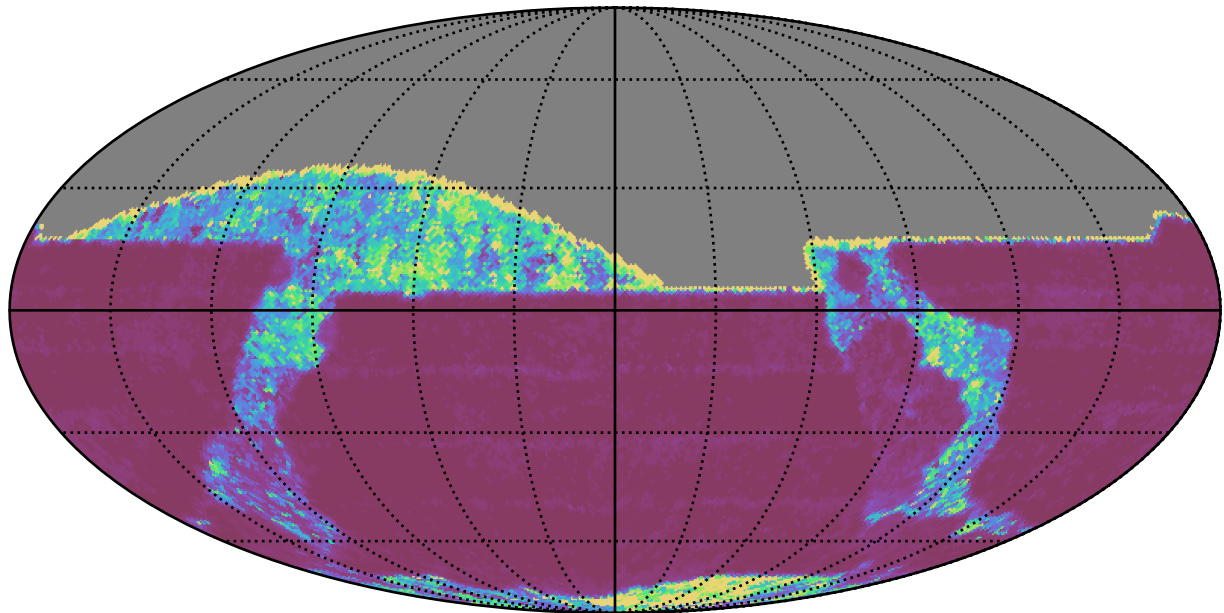
early_u_fpextra2.0_v3.4_10yrs All sky z band: 20thPercentile Inter-Night Gap
