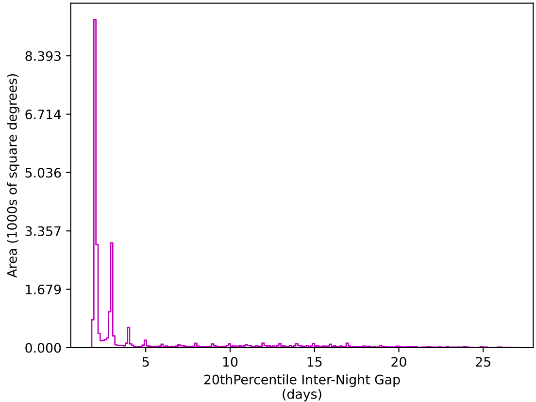
early_u_fpextra2.0_v3.4_10yrs All sky z band: 20thPercentile Inter-Night Gap
