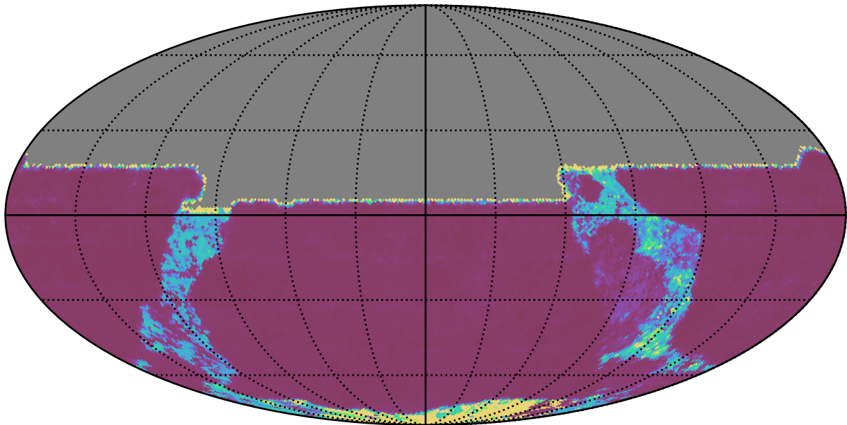
early_u_fpextra2.0_v3.4_10yrs All sky y band: 20thPercentile Inter-Night Gap
