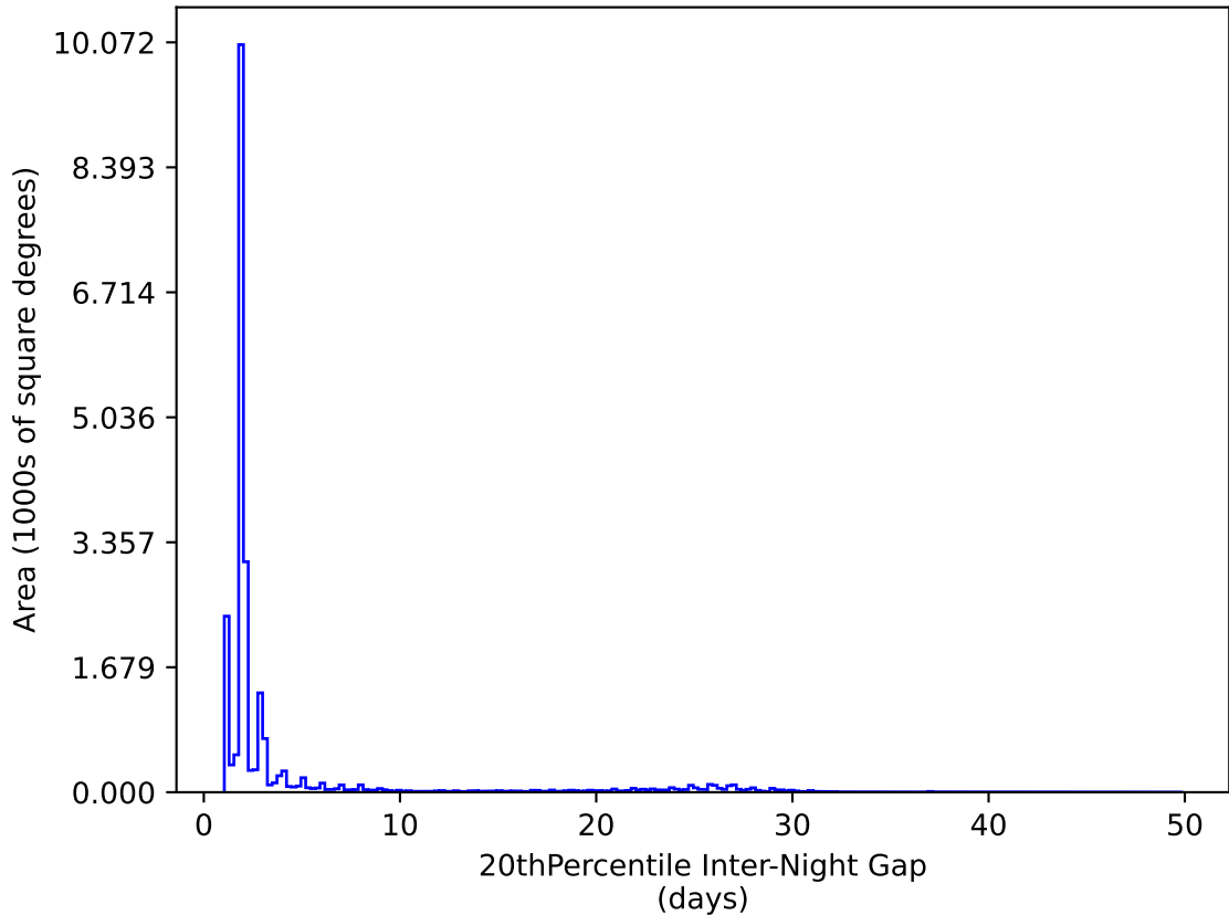
early_u_fpextra2.0_v3.4_10yrs All sky y band: 20thPercentile Inter-Night Gap
