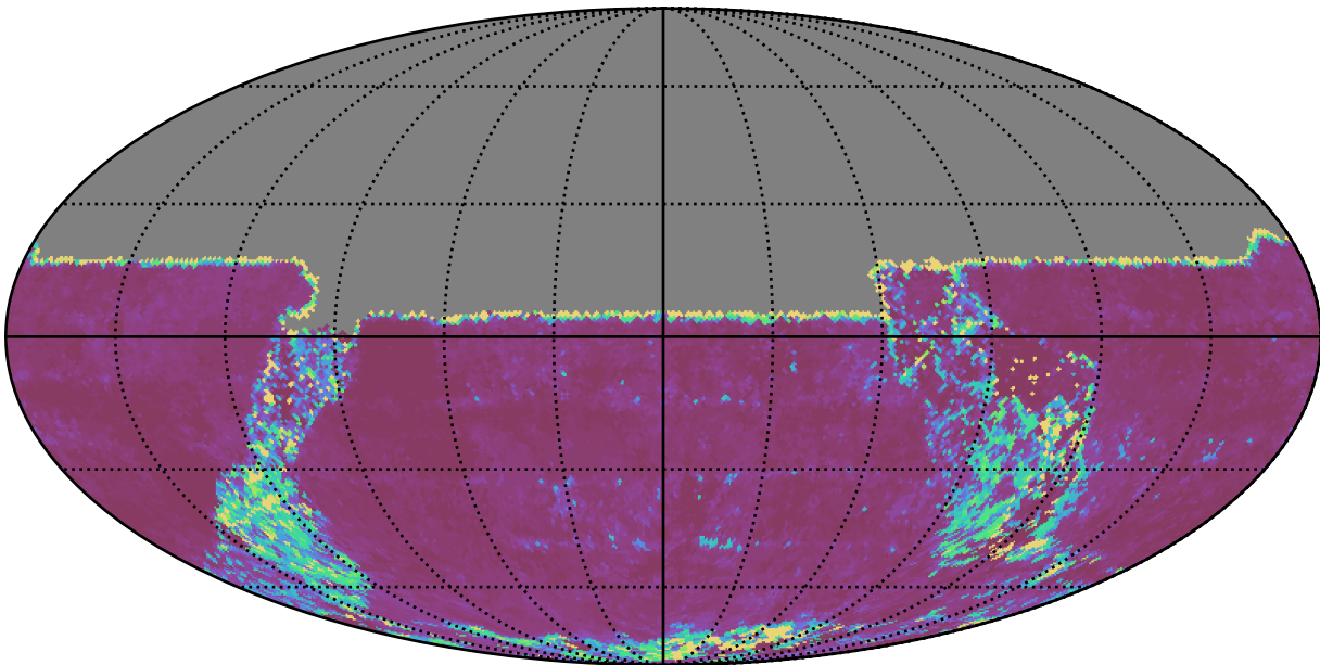
early_u_fpextra2.0_v3.4_10yrs All sky u band: 20thPercentile Inter-Night Gap
