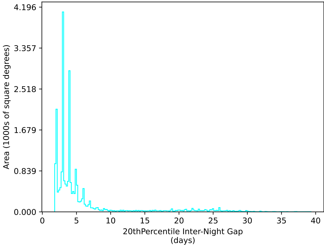
early_u_fpextra2.0_v3.4_10yrs All sky u band: 20thPercentile Inter-Night Gap
