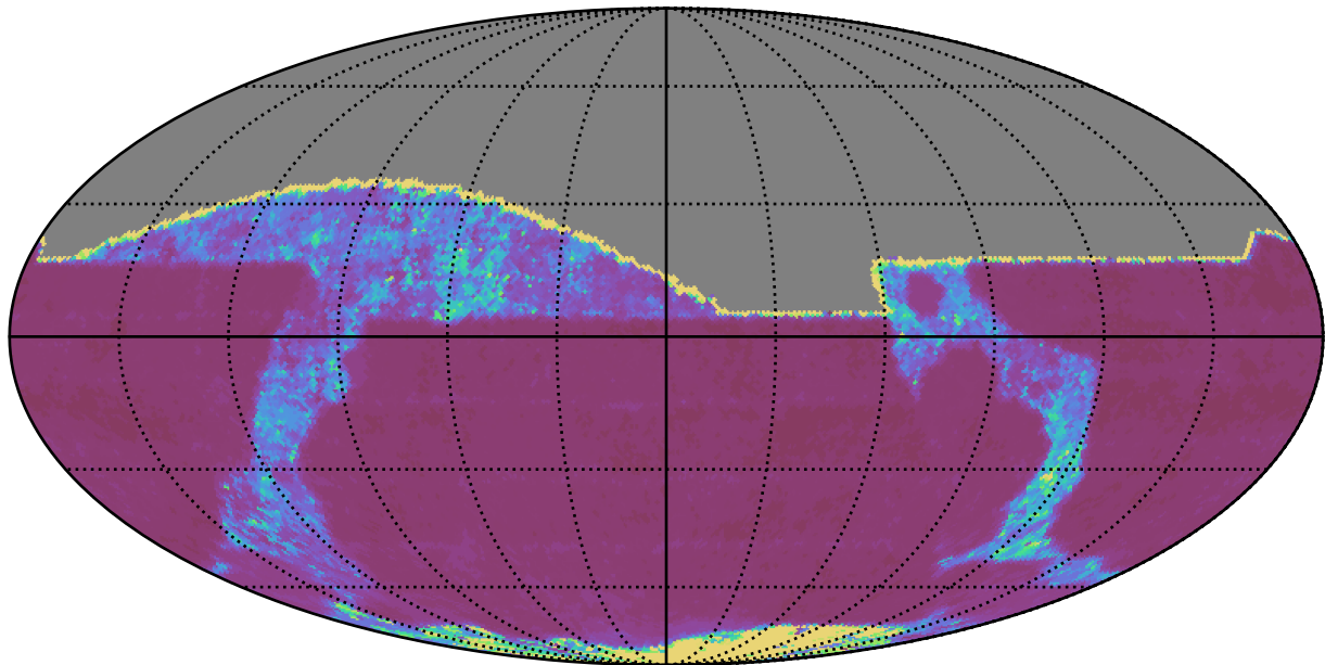
early_u_fpextra2.0_v3.4_10yrs All sky r band: 20thPercentile Inter-Night Gap
