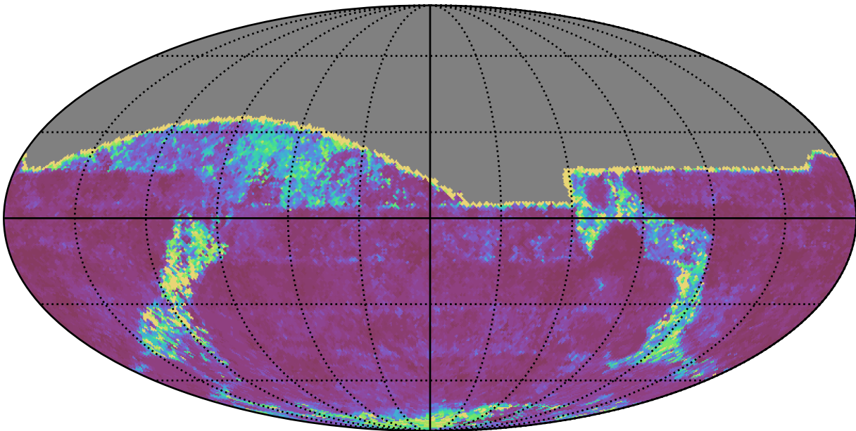
early_u_fpextra2.0_v3.4_10yrs All sky g band: 20thPercentile Inter-Night Gap
