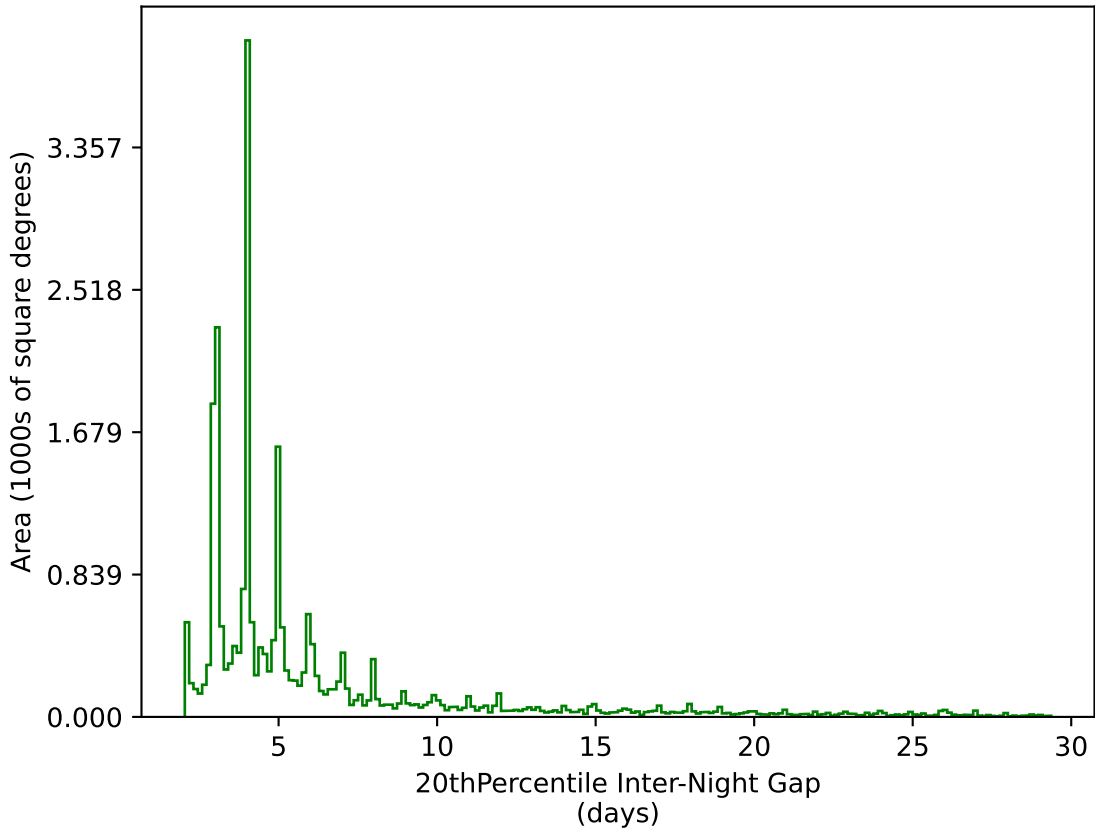
early_u_fpextra2.0_v3.4_10yrs All sky g band: 20thPercentile Inter-Night Gap
