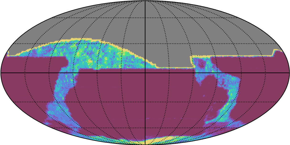
early_u_fpextra2.0_v3.4_10yrs All sky all bands: 20thPercentile Inter-Night Gap
