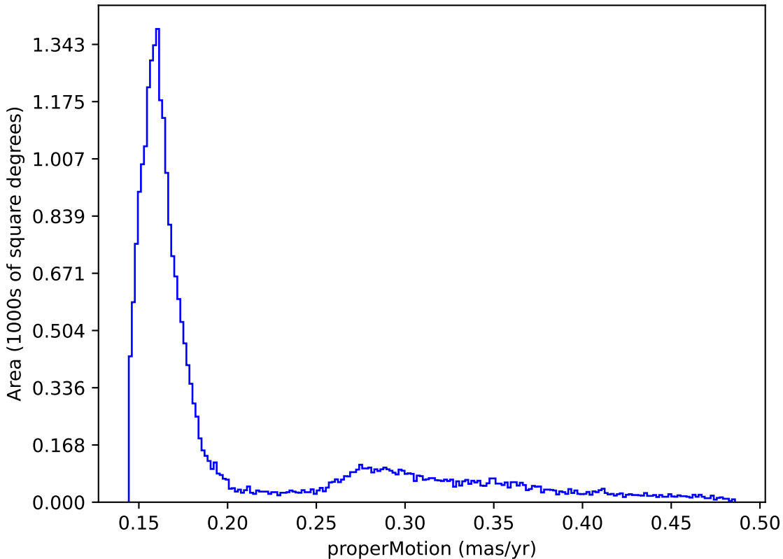
early_u_fpextra2.0_v3.4_10yrs : properMotion
