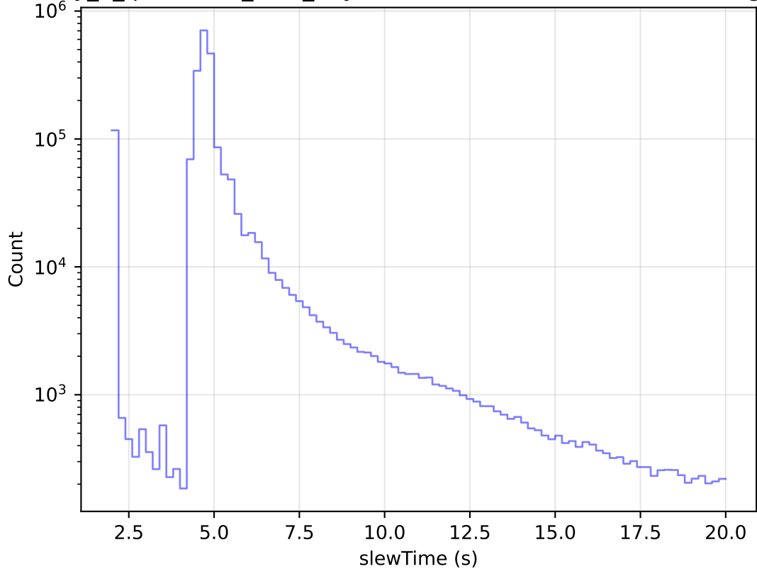
early_u_fpextra2.0_v3.4_10yrs All visits: Zoom Slew Time Histogram
