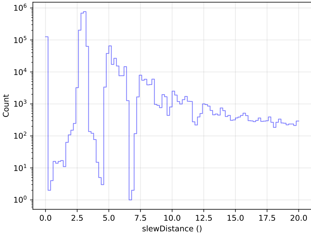
early_u_fpextra2.0_v3.4_10yrs All visits: Zoom Slew Distance Histogram
