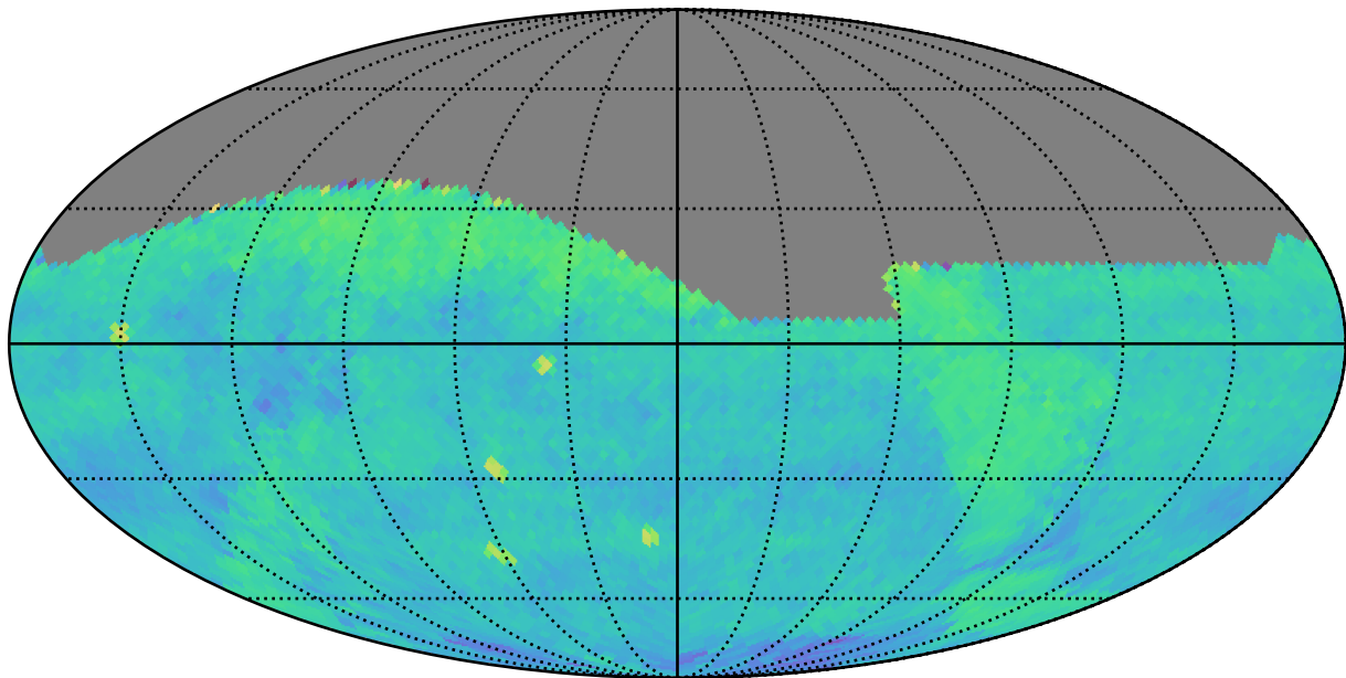
early_u_fpextra2.0_v3.4_10yrs (g or r or i): PairFraction
