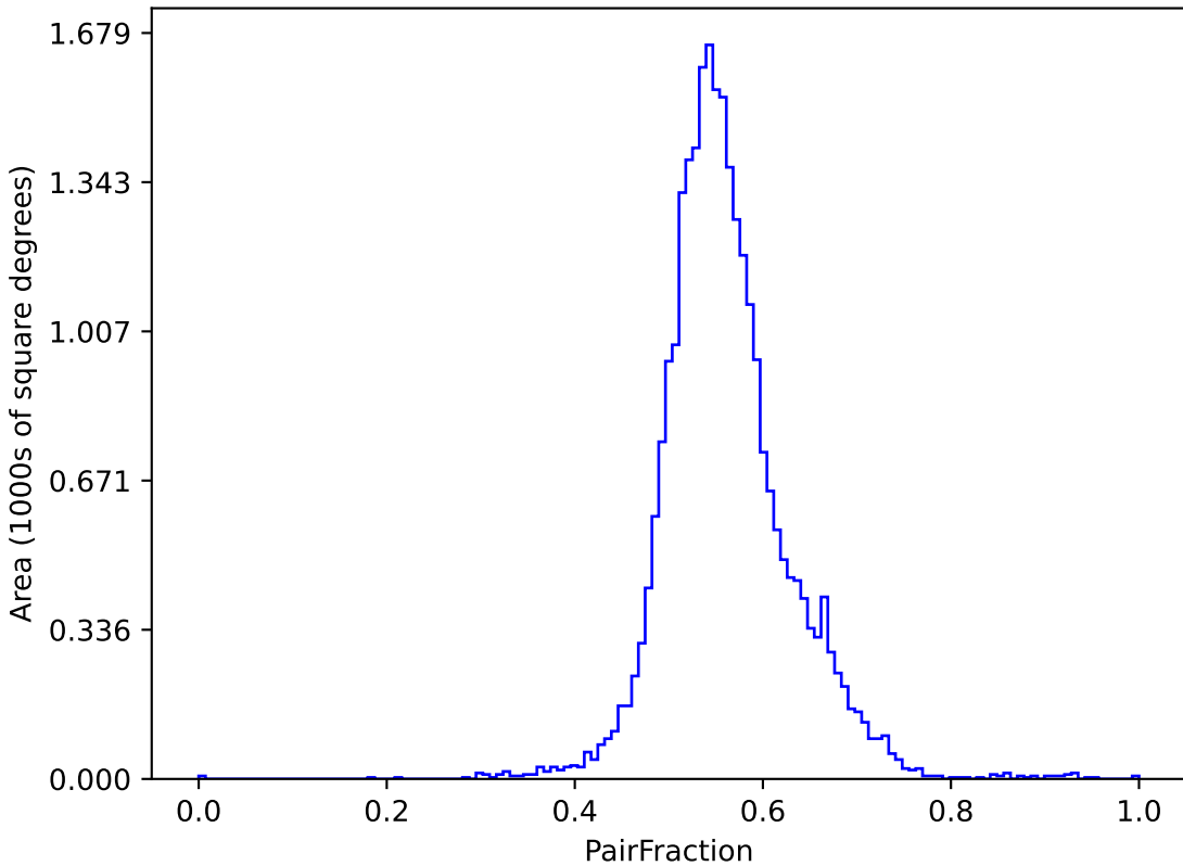
early_u_fpextra2.0_v3.4_10yrs (g or r or i): PairFraction
