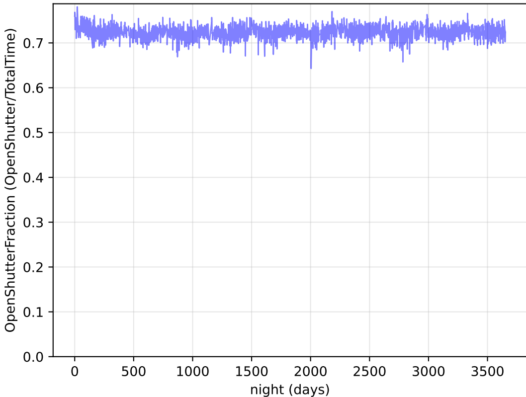
early_u_fpextra2.0_v3.4_10yrs : OpenShutterFraction
