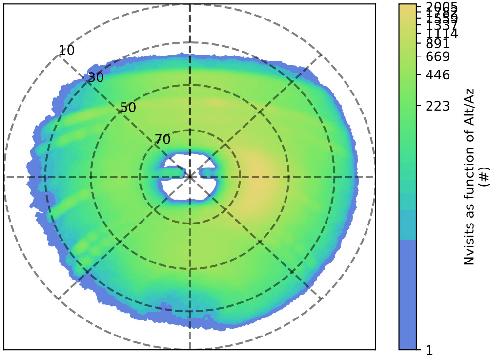
early_u_fpextra2.0_v3.4_10yrs y: Nvisits as function of Alt/Az
