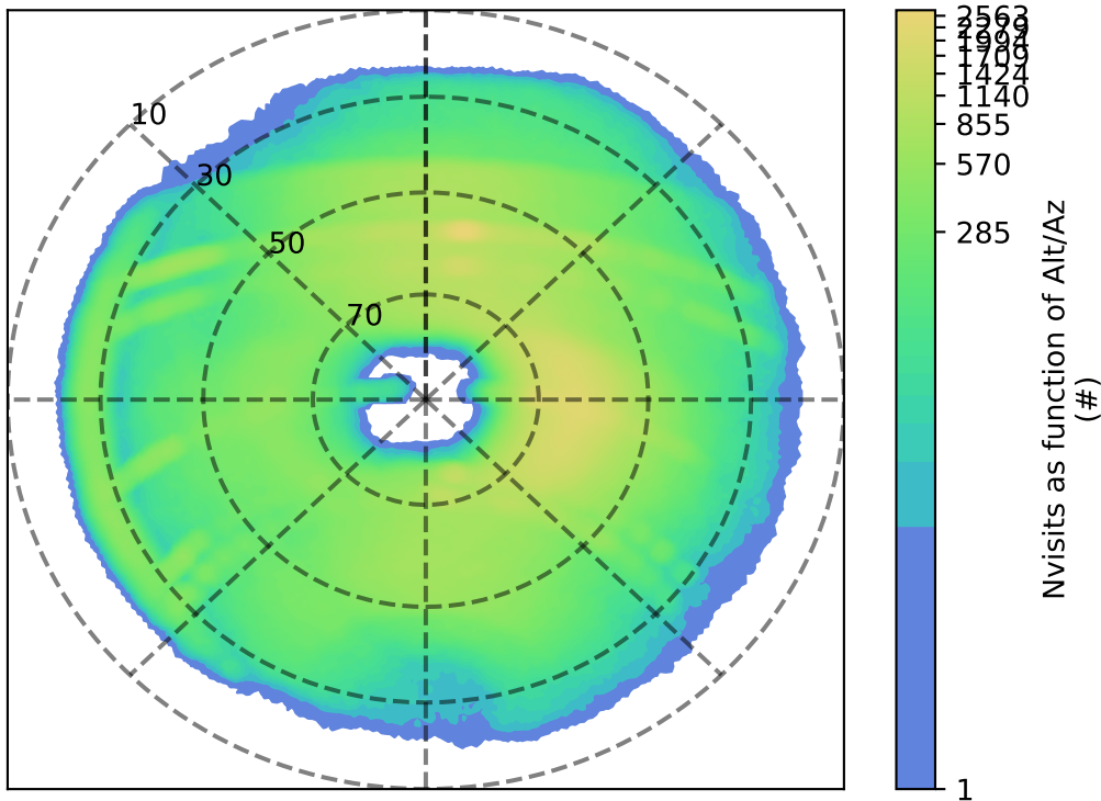
early_u_fpextra2.0_v3.4_10yrs r: Nvisits as function of Alt/Az
