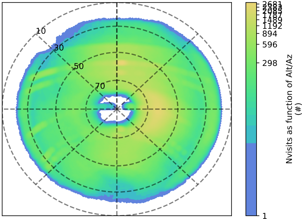
early_u_fpextra2.0_v3.4_10yrs i: Nvisits as function of Alt/Az
