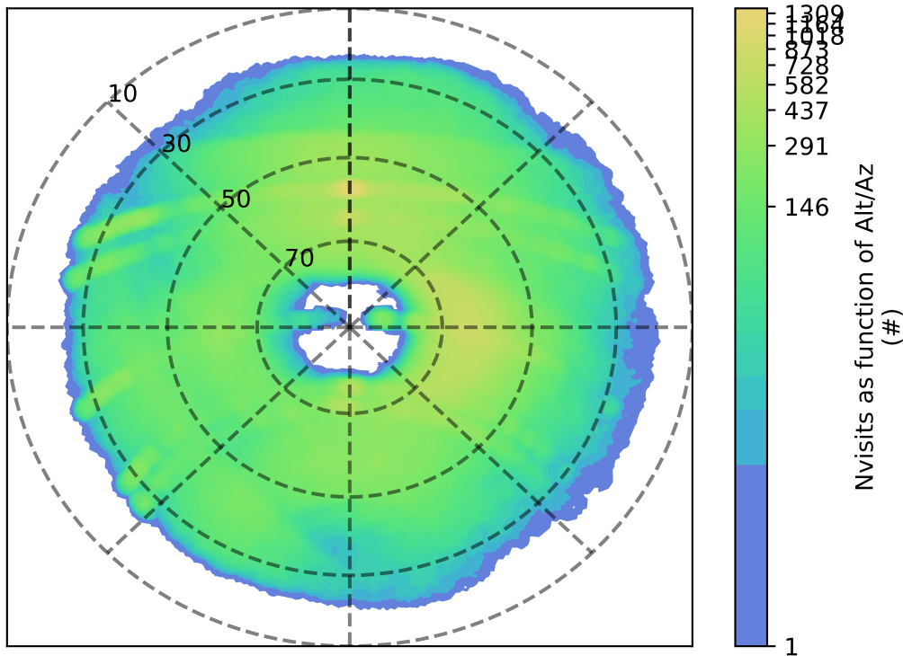
early_u_fpextra2.0_v3.4_10yrs g: Nvisits as function of Alt/Az
