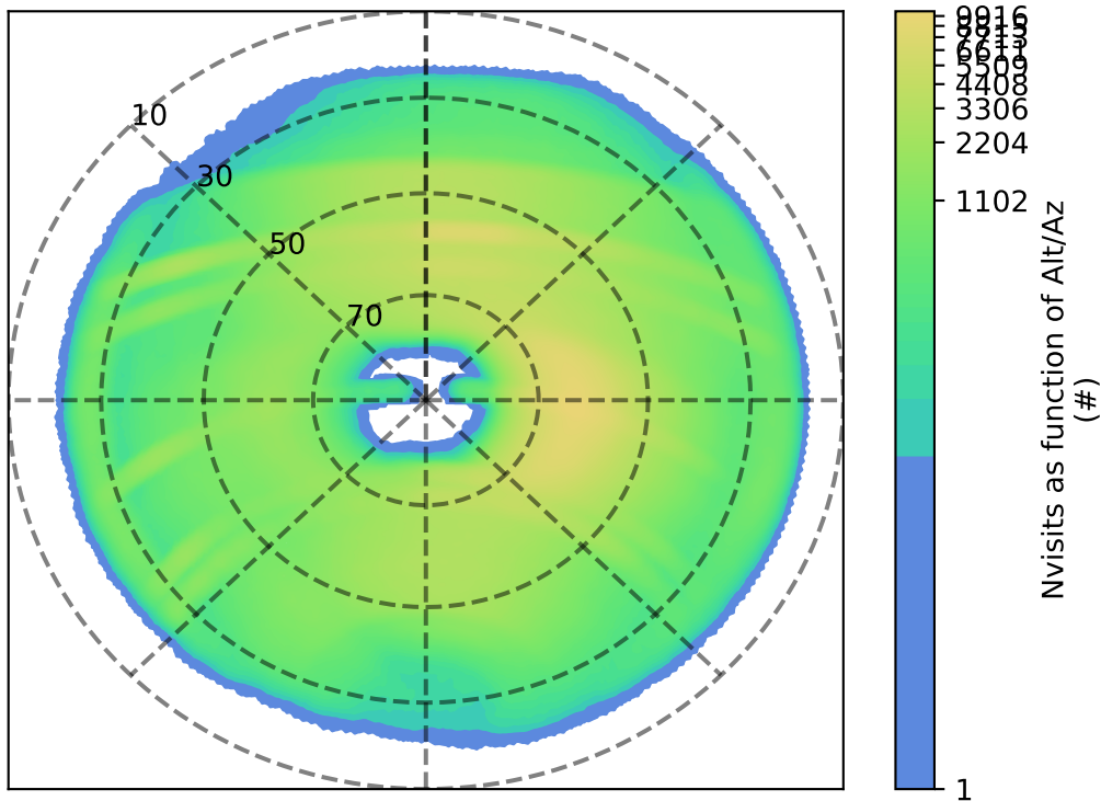
early_u_fpextra2.0_v3.4_10yrs : Nvisits as function of Alt/Az
