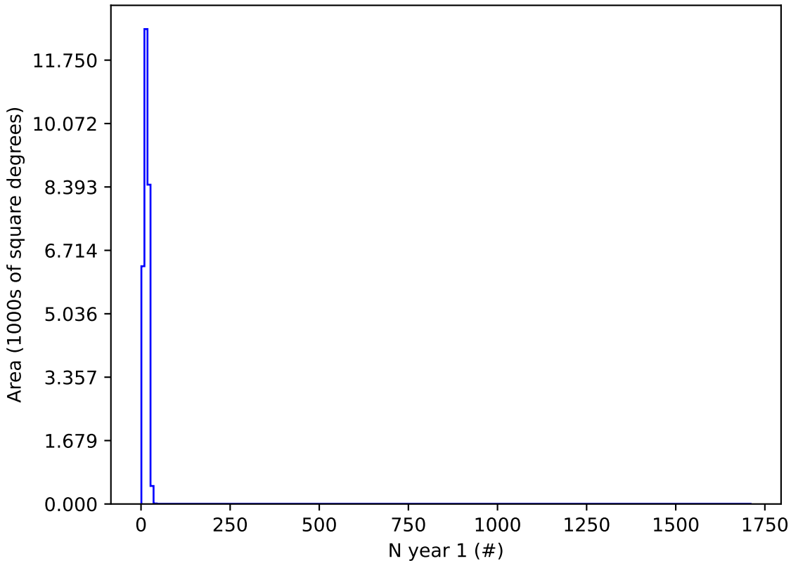
early_u_fpextra2.0_v3.4_10yrs r and night < 365: N year 1
