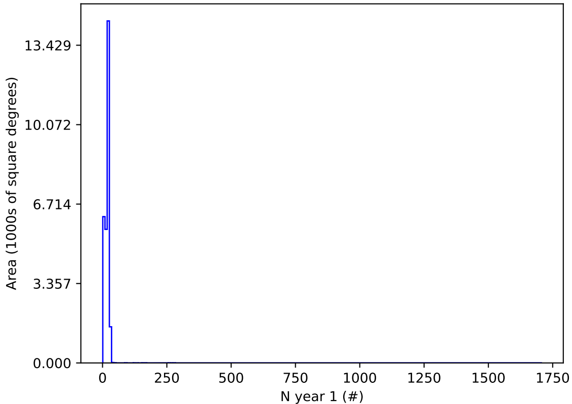
early_u_fpextra2.0_v3.4_10yrs i and night < 365: N year 1
