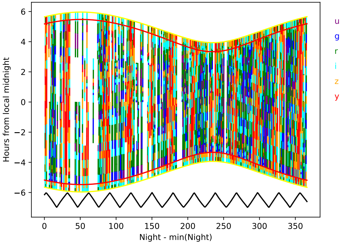
early_u_fpextra2.0_v3.4_10yrs year 9-10: Hourglass
