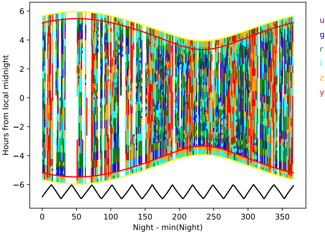
early_u_fpextra2.0_v3.4_10yrs year 8-9: Hourglass
