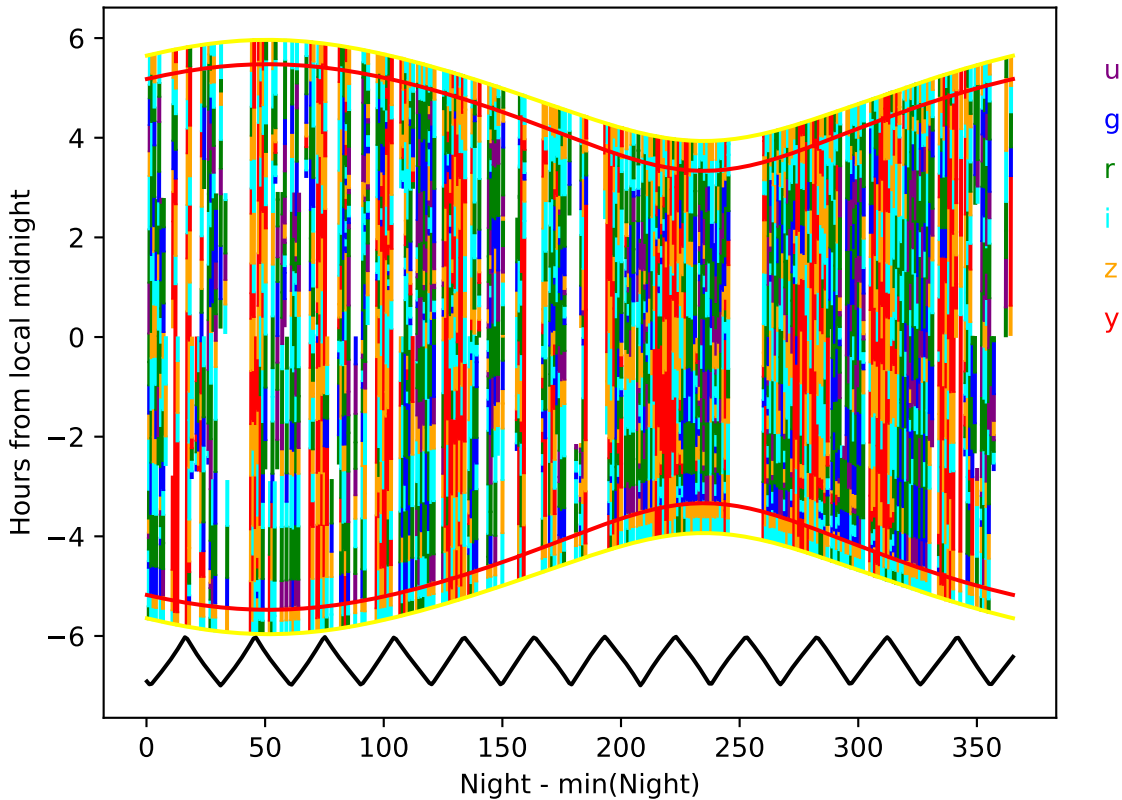
early_u_fpextra2.0_v3.4_10yrs year 5-6: Hourglass
