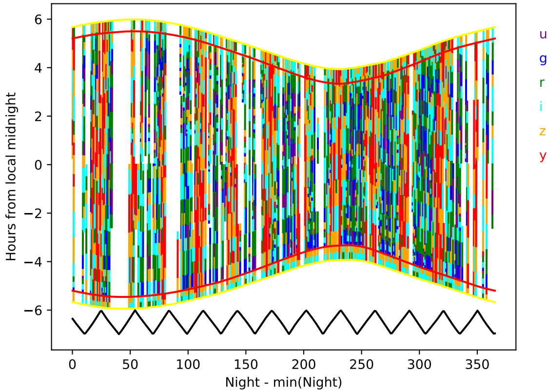
early_u_fpextra2.0_v3.4_10yrs year 4-5: Hourglass
