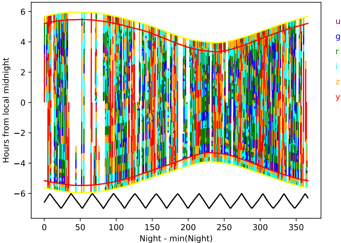
early_u_fpextra2.0_v3.4_10yrs year 3-4: Hourglass
