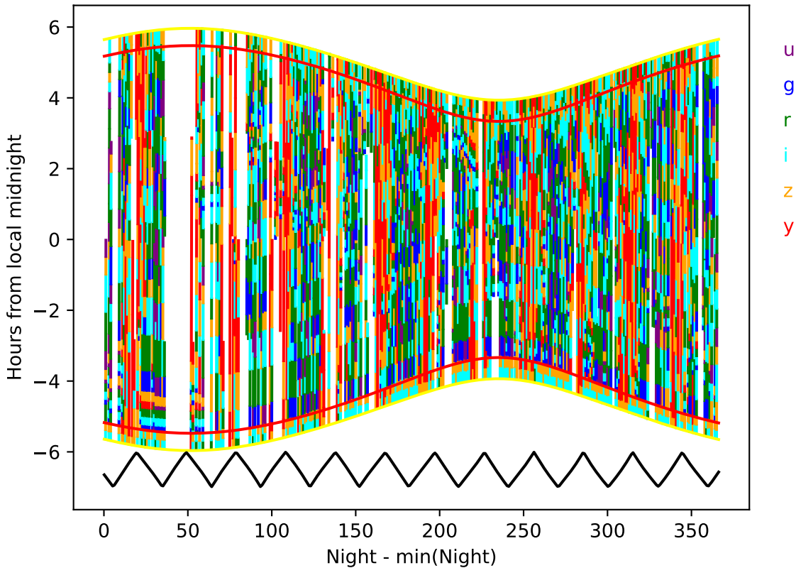
early_u_fpextra2.0_v3.4_10yrs year 2-3: Hourglass
