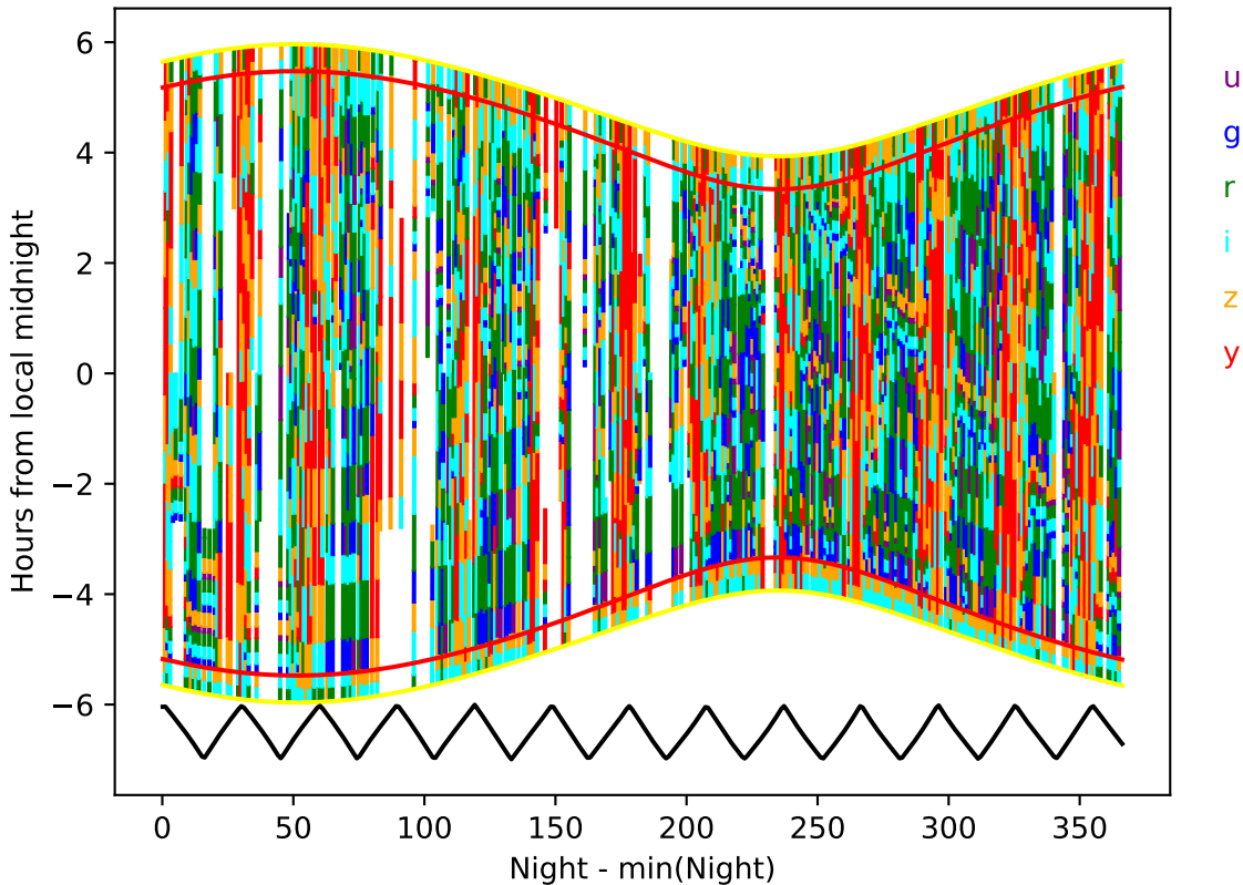
early_u_fpextra2.0_v3.4_10yrs year 1-2: Hourglass
