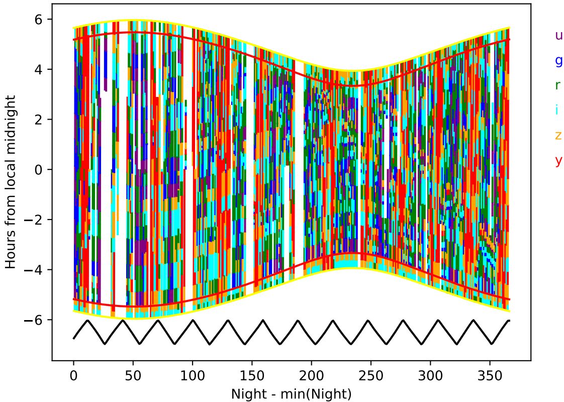
early_u_fpextra2.0_v3.4_10yrs year 0-1: Hourglass
