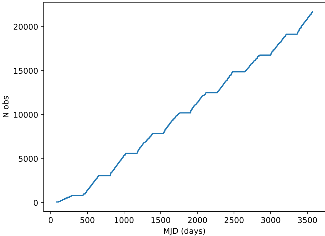
early_u_fpextra2.0_v3.4_10yrs note like DD:XMM_LSS%: Cumulative
