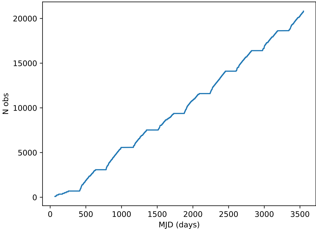
early_u_fpextra2.0_v3.4_10yrs note like DD:ELAISS1%: Cumulative
