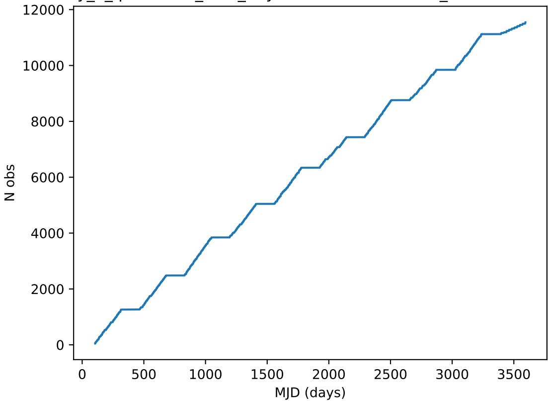
early_u_fpextra2.0_v3.4_10yrs note like DD:EDFS_a%: Cumulative
