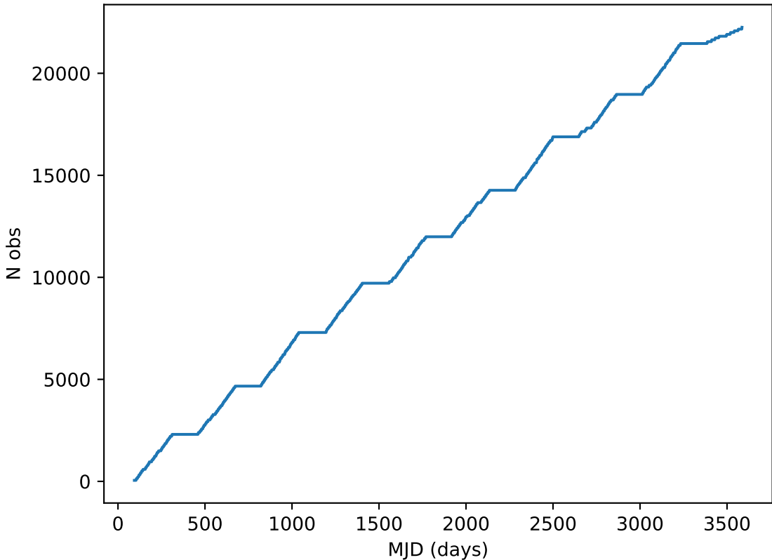
early_u_fpextra2.0_v3.4_10yrs note like DD:ECDFS%: Cumulative
