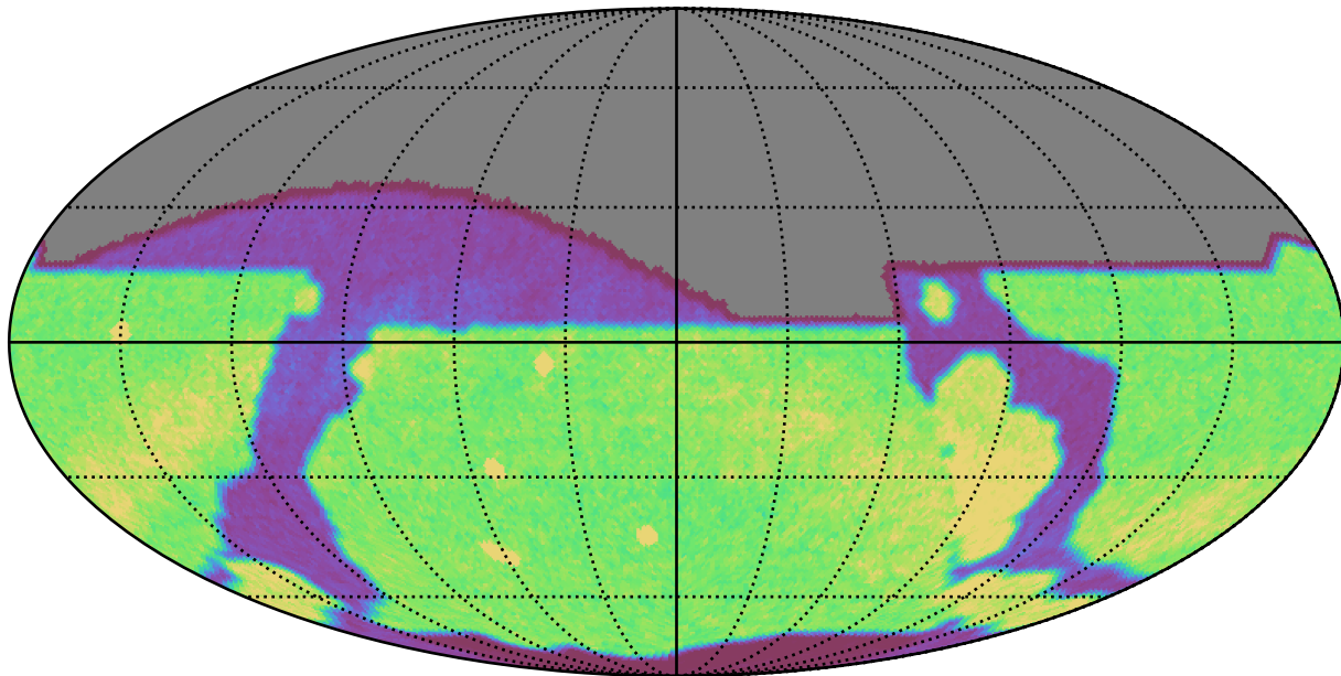
early_u_fpextra2.0_v3.4_10yrs r: Count observationStartMJD
